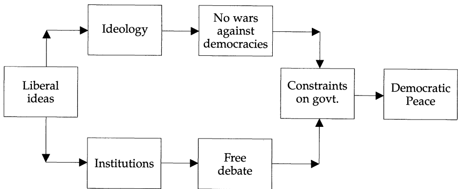
Figure 1. Causal Pathways of Liberal Democratic Peace.
