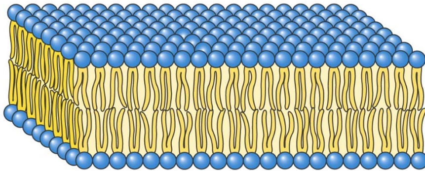
Bilayer (b)
