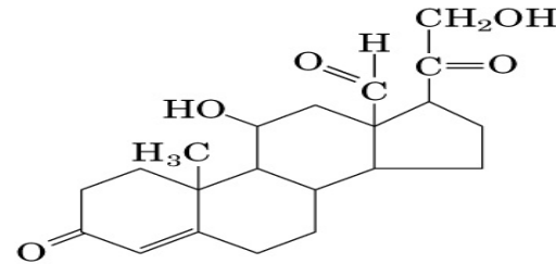
Aldosterone
