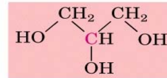
Glycerol
