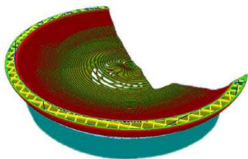
Fig. 11: Preparatory slicing to 3D printing
