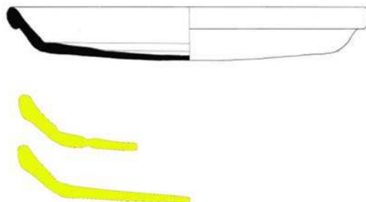
Fig. 10: Comparison between the section of the traditional survey and sections obtained from polygonal mesh (N.I. 48251).
