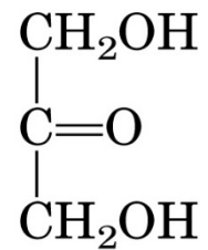
Dihydroxyacetone
