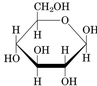
\beta -D-Glucopyranose
