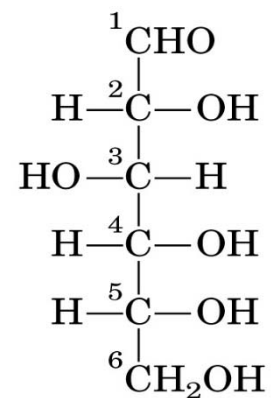
D-Glucose
