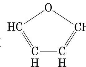
Furan
