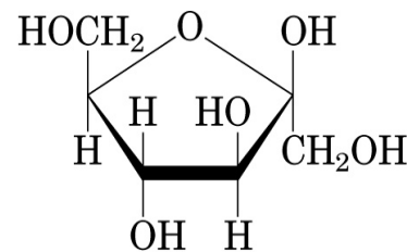
\beta -D-Fructofuranose
