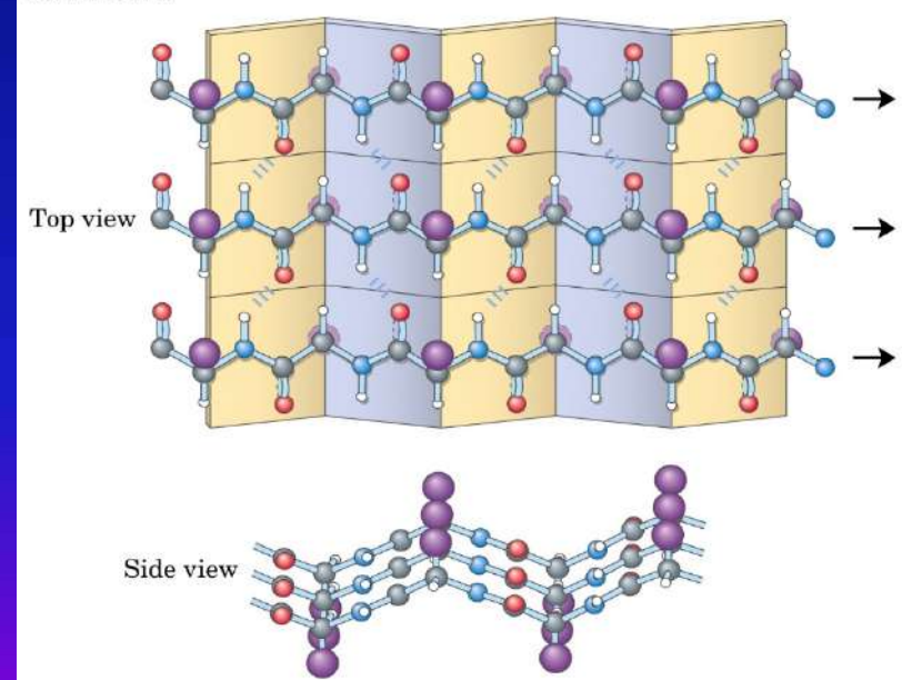
(b) Parallelo
