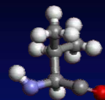
Val
