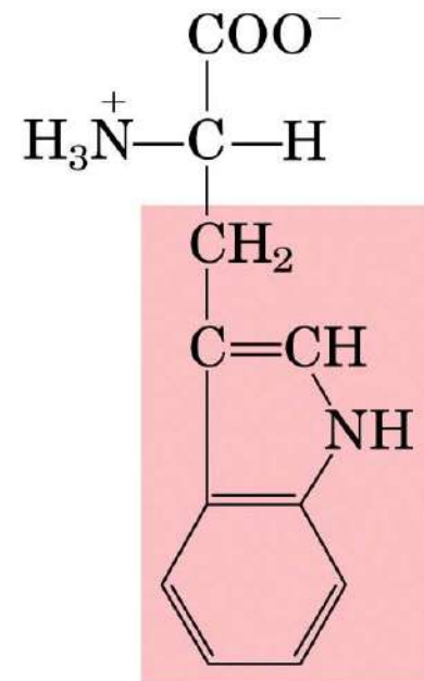
Tryptophan
