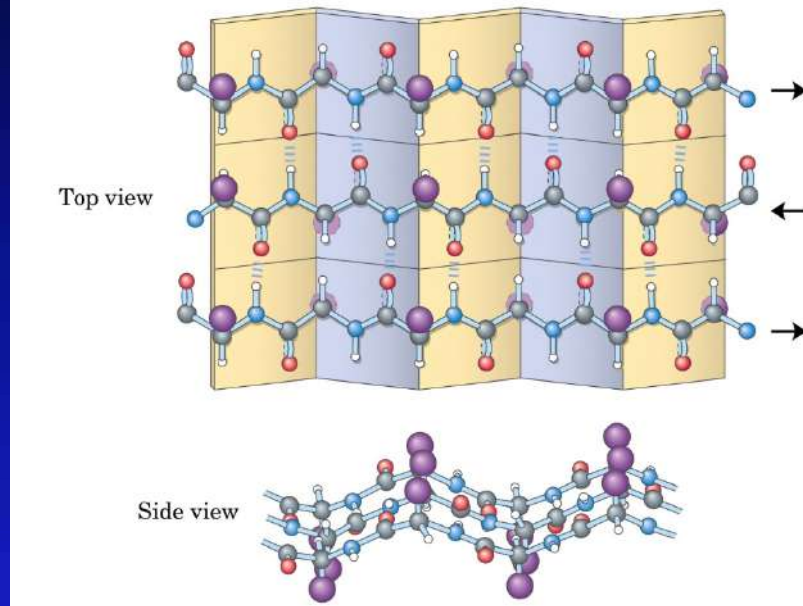
(a) Antiparallelo
