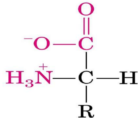
Zwitterionic form
