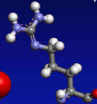
Arg
