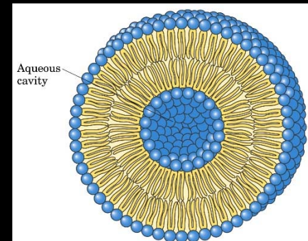
Liposome (c)
