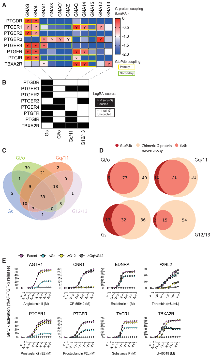
Figure 3. Comparison of G-Protein Coupling between the Chimeric G-Protein-Based Assay and GtoPdb, and Validation of G 12/13 Signaling for the Newly Characterized GPCRs
