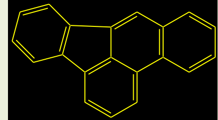
Benzo[b]fluorantene
