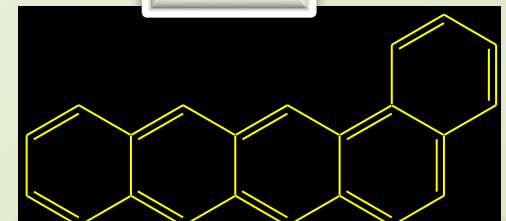
dibenzo[a,h]antracene
