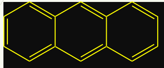
antracene
