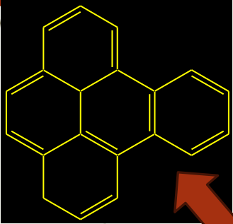
Benzo[e]pirene
