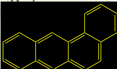
Benzo[a]antracene
